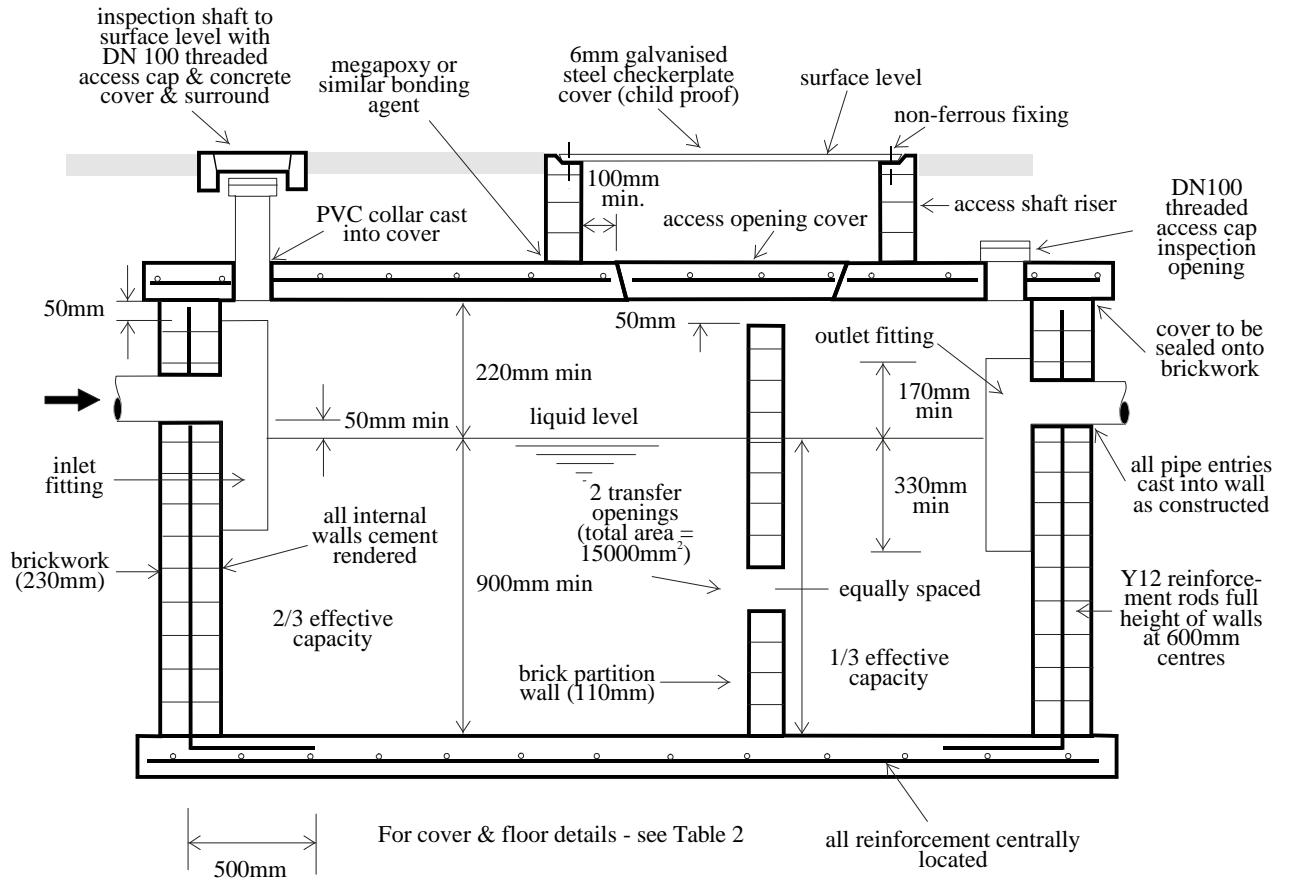
FIGURE 6: RECTANGULAR BRICK SEPTIC TANK
